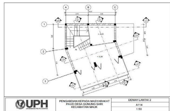
Gambar 6. 6 Denah Lantai 2
